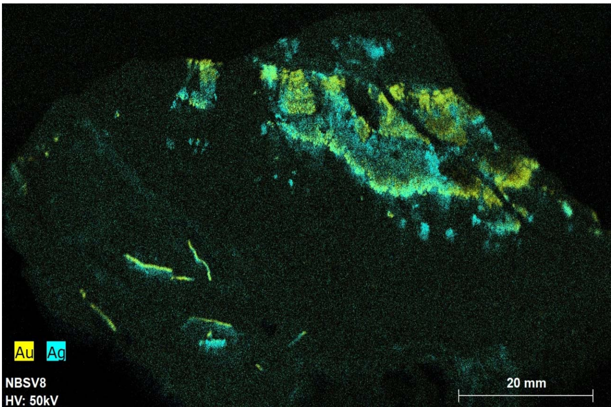
Micro XRF image of sample PR 1420 showing strong association of high-grade gold and silver with sulphidic 'ginguro'.
