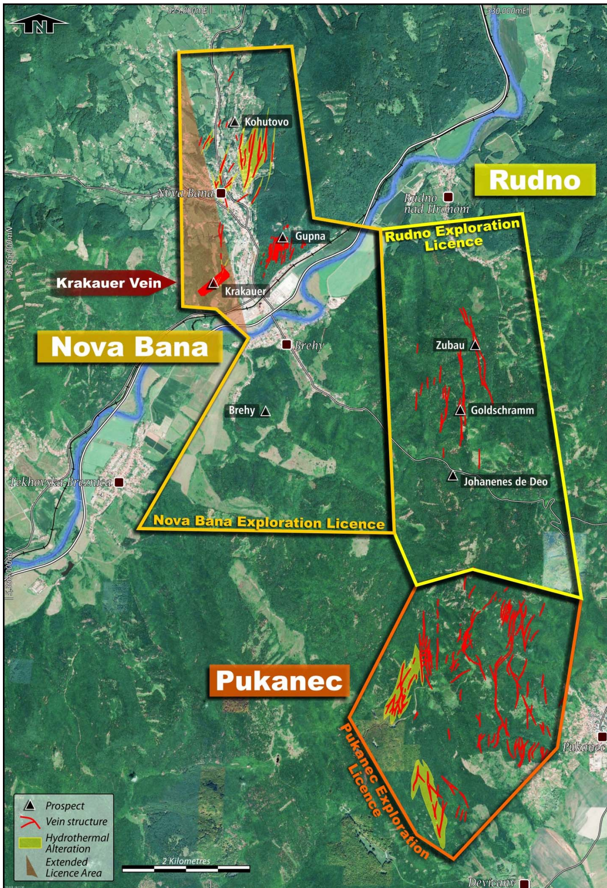
Prospech's western exploration licences showing the extended Nova Bana area and the location of the Krakauer discovery.
